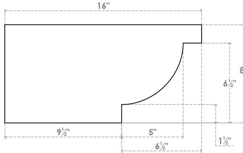
SIDE PROFILE
